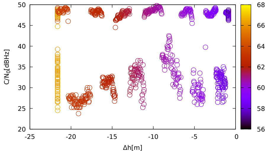
C/N 0 vs height (TrimbleR10 (down) for G26 at L1)
