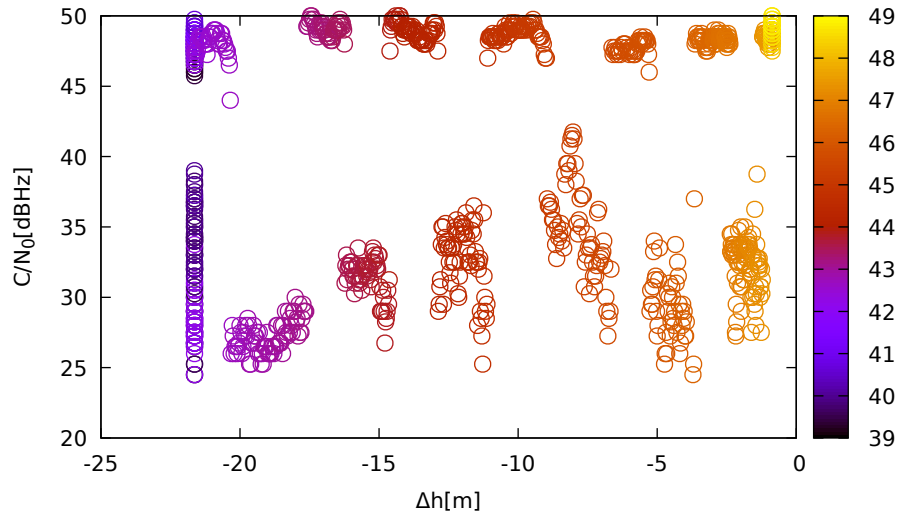
C/N 0 vs height (TrimbleR10 (down) for G29 at L1)
