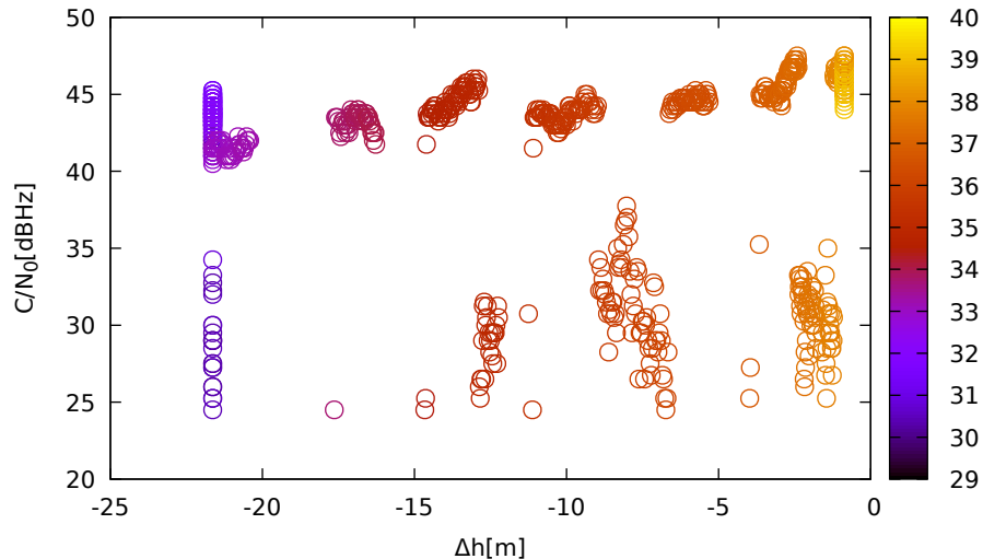
C/N 0 vs height (TrimbleR10 (down) for G31 at L1)
