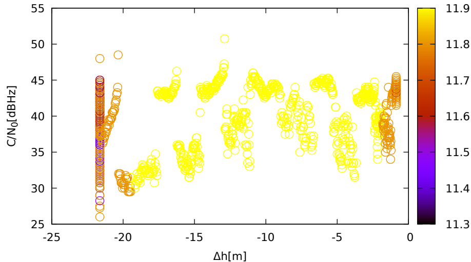
C/N 0 vs height (TrimbleR10 (down) for R02 at L1)
