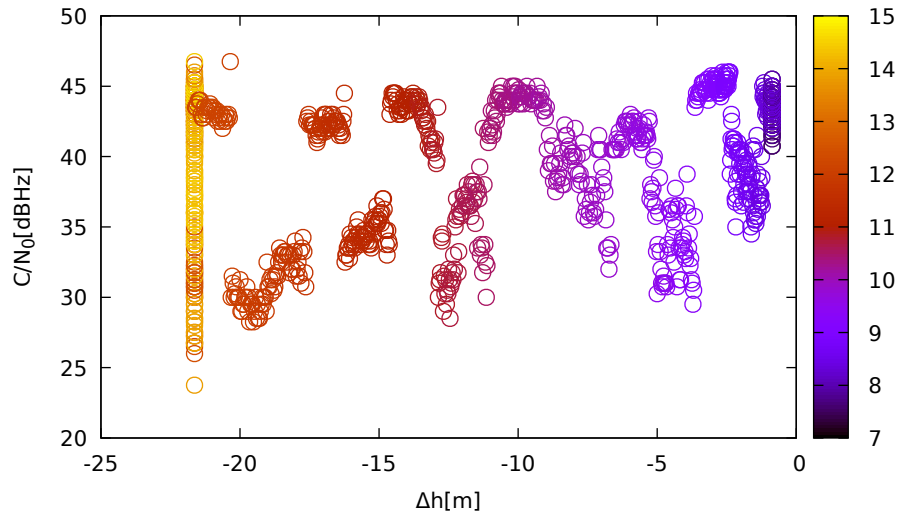
C/N 0 vs height (TrimbleR10 (down) for R03 at L1)
