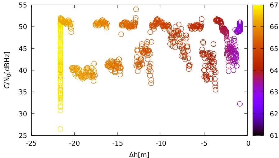
C/N 0 vs height (TrimbleR10 (down) for R09 at L1)
