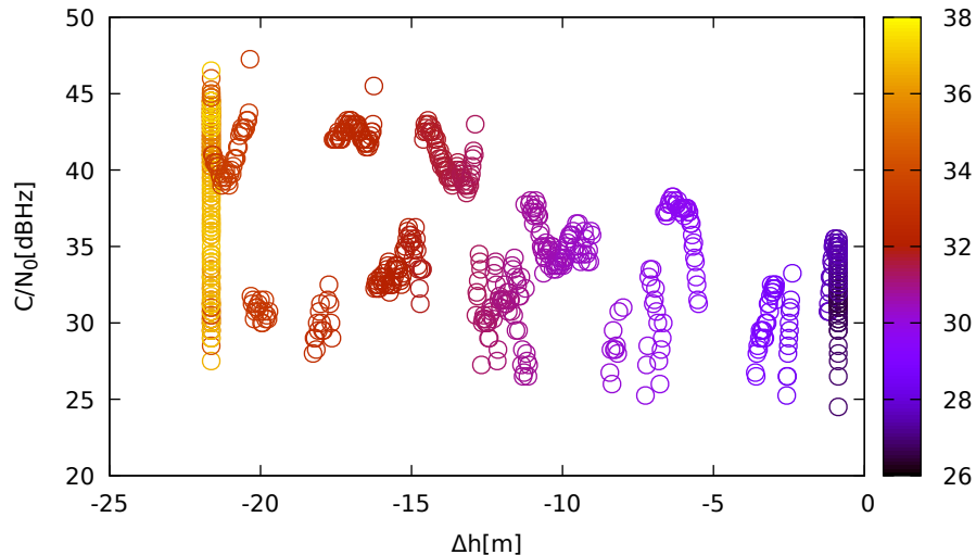
C/N 0 vs height (TrimbleR10 (down) for R10 at L1)
