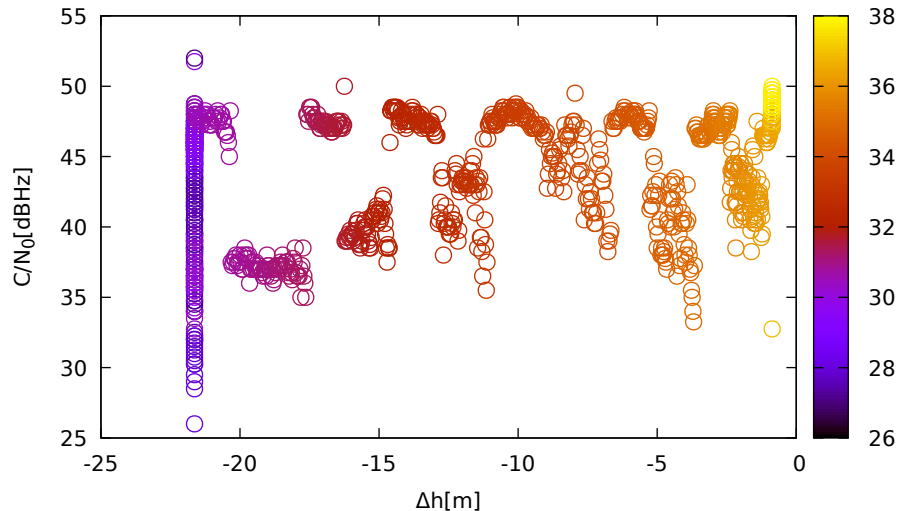
C/N 0 vs height (TrimbleR10 (down) for R18 at L1)
