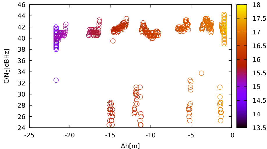
C/N 0 vs height (TrimbleR8s (down) for G05 at L1)
