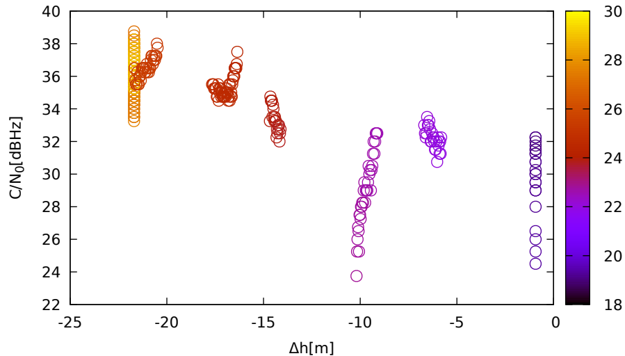
C/N 0 vs height (TrimbleR8s (down) for G16 at L1)
