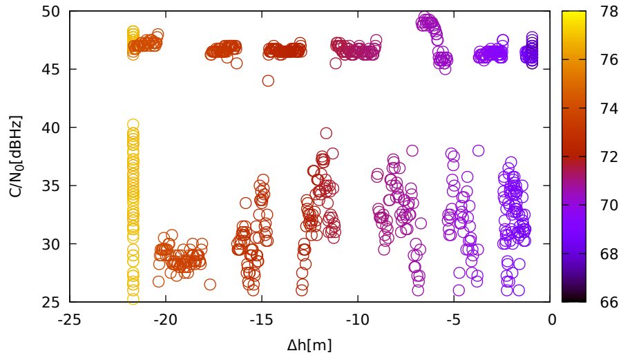
C/N 0 vs height (TrimbleR8s (down) for G18 at L1)
