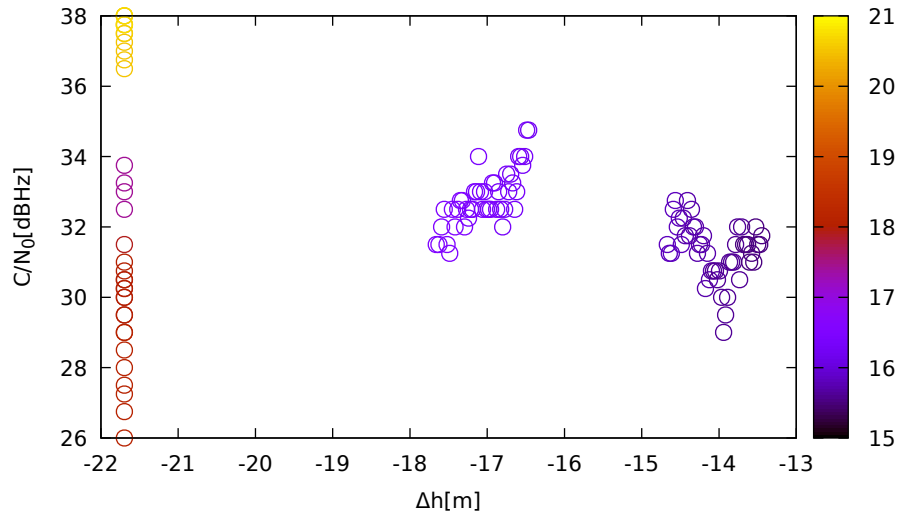
C/N 0 vs height (TrimbleR8s (down) for G20 at L1)
