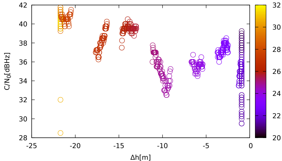
C/N 0 vs height (TrimbleR8s (down) for G21 at L1)
