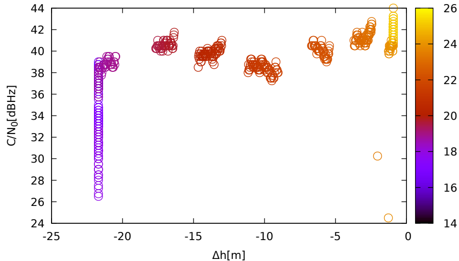
C/N 0 vs height (TrimbleR8s (down) for G25 at L1)
