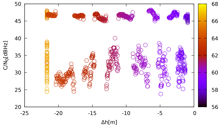
C/N 0 vs height (TrimbleR8s (down) for G26 at L1)
