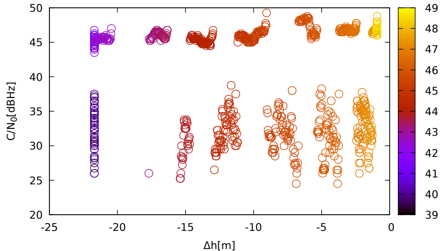
C/N 0 vs height (TrimbleR8s (down) for G29 at L1)
