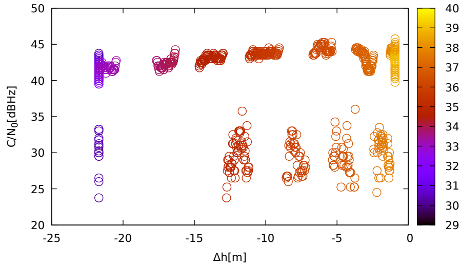
C/N 0 vs height (TrimbleR8s (down) for G31 at L1)
