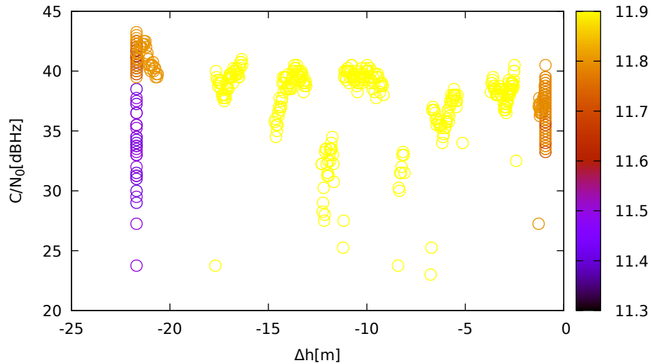
C/N 0 vs height (TrimbleR8s (down) for R02 at L1)
