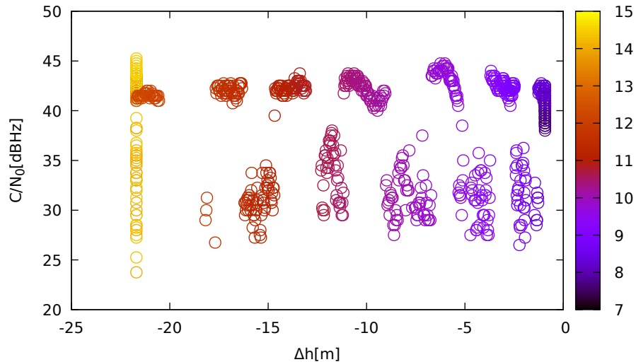
C/N 0 vs height (TrimbleR8s (down) for R03 at L1)
