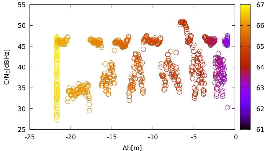
C/N 0 vs height (TrimbleR8s (down) for R09 at L1)
