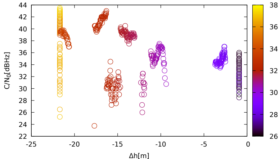
C/N 0 vs height (TrimbleR8s (down) for R10 at L1)
