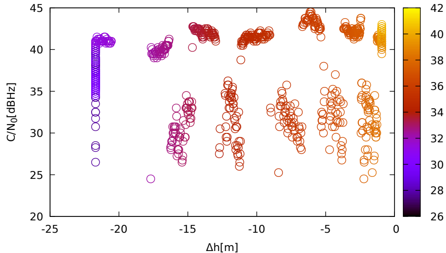
C/N 0 vs height (TrimbleR8s (down) for R16 at L1)
