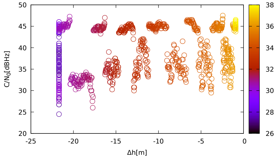
C/N 0 vs height (TrimbleR8s (down) for R18 at L1)
