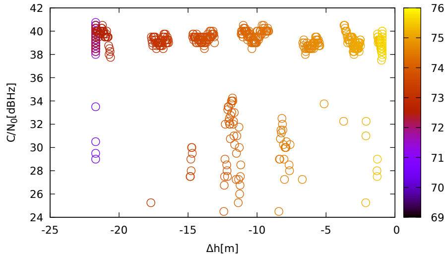
C/N 0 vs height (TrimbleR8s (down) for R19 at L1)
