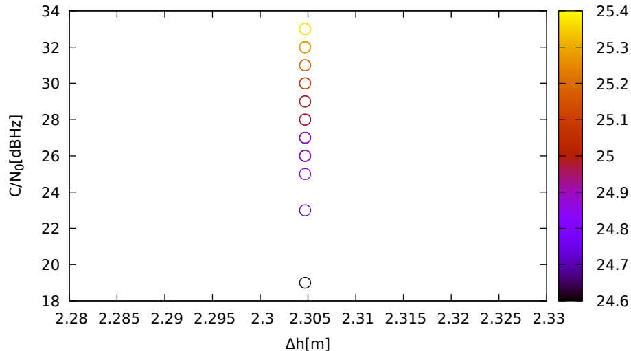
C/N 0 vs height (ublox9 (down) for E01 at L1)
