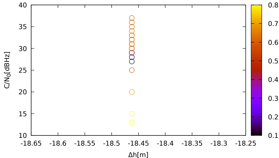
C/N 0 vs height (ublox9 (down) for E07 at L1)
