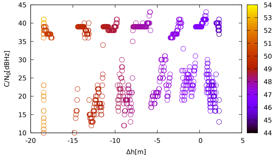
C/N 0 vs height (ublox9 (down) for E12 at L1)
