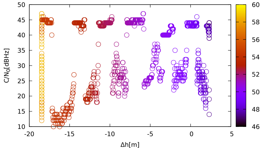
C/N 0 vs height (ublox9 (down) for E18 at L1)
