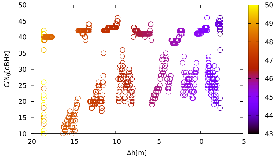
C/N 0 vs height (ublox9 (down) for E24 at L1)
