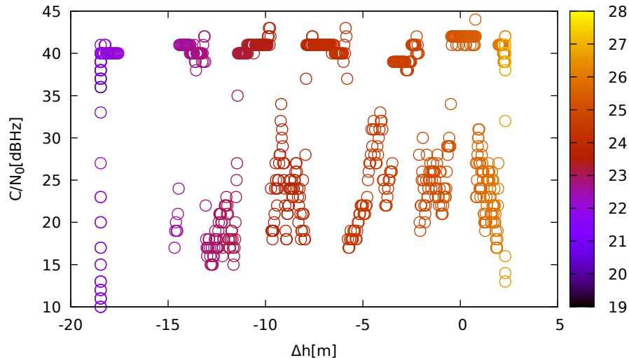
C/N 0 vs height (ublox9 (down) for E26 at L1)
