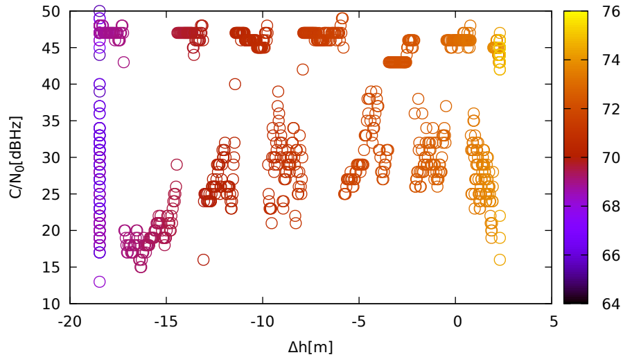
C/N 0 vs height (ublox9 (down) for E31 at L1)
