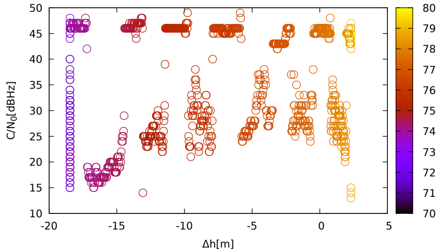
C/N 0 vs height (ublox9 (down) for E33 at L1)
