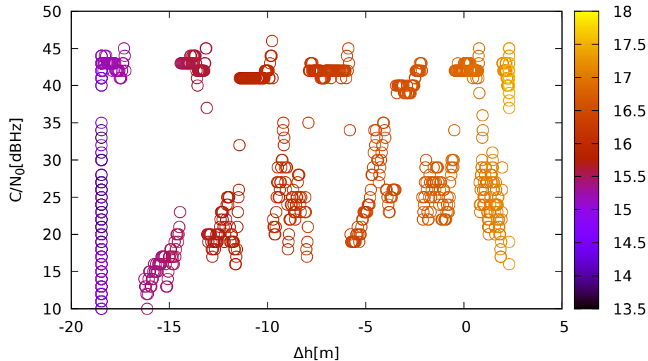
C/N 0 vs height (ublox9 (down) for G05 at L1)
