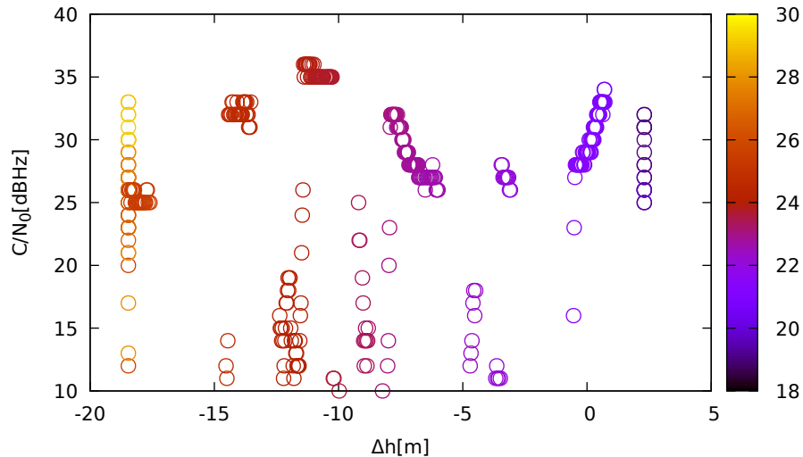
C/N 0 vs height (ublox9 (down) for G16 at L1)
