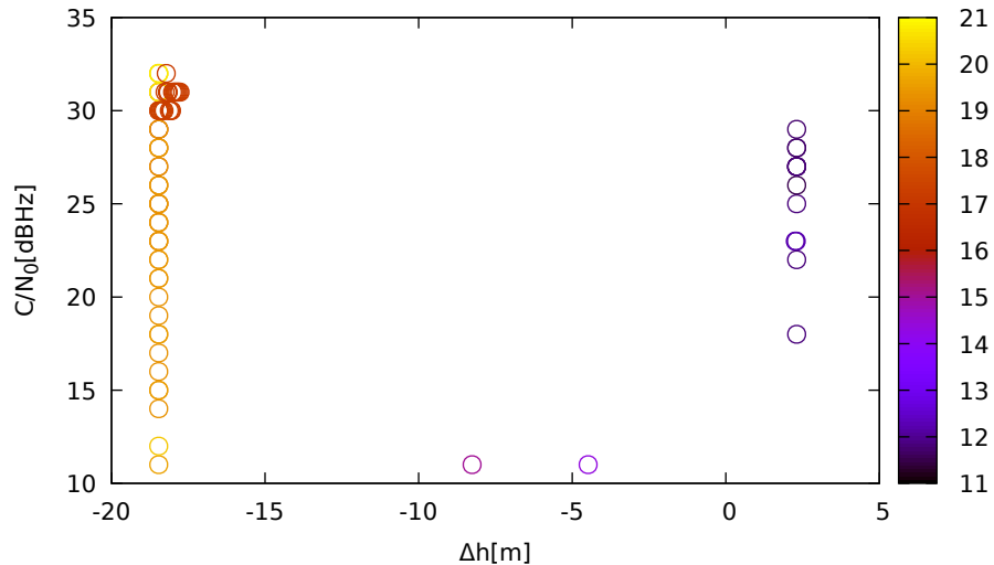
C/N 0 vs height (ublox9 (down) for G20 at L1)
