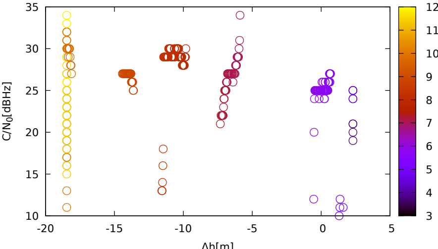
C/N 0 vs height (ublox9 (down) for G23 at L1)
