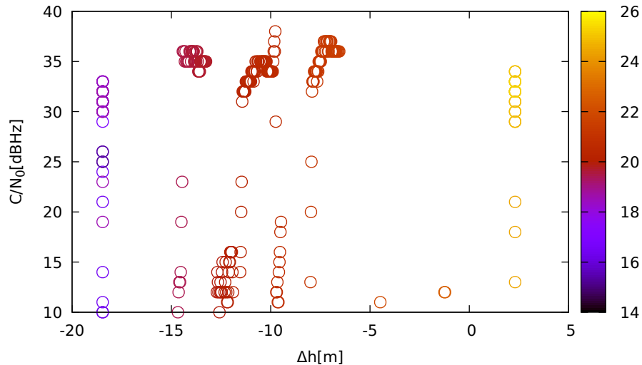
C/N 0 vs height (ublox9 (down) for G25 at L1)
