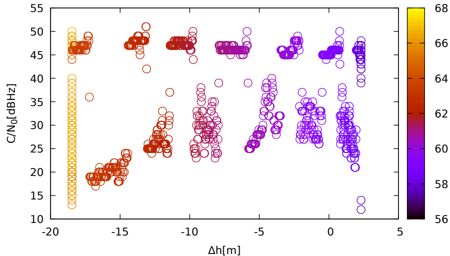
C/N 0 vs height (ublox9 (down) for G26 at L1)
