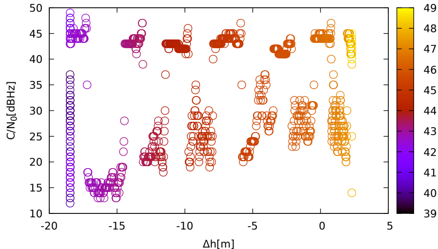
C/N 0 vs height (ublox9 (down) for G29 at L1)
