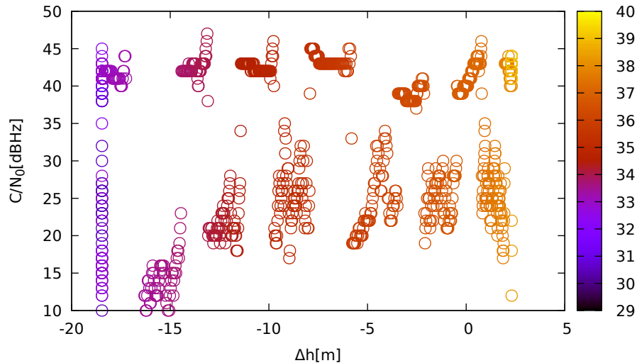
C/N 0 vs height (ublox9 (down) for G31 at L1)
