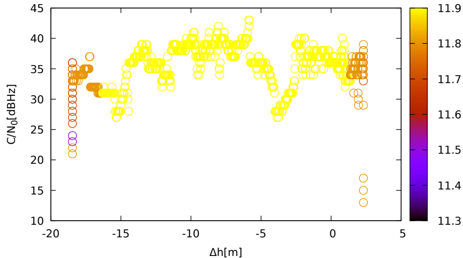
C/N 0 vs height (ublox9 (down) for R02 at L1)
