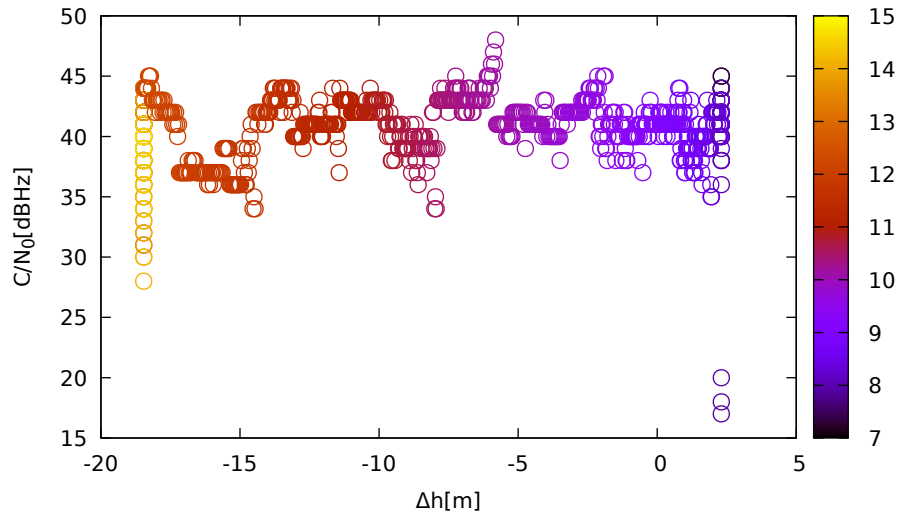
C/N 0 vs height (ublox9 (down) for R03 at L1)
