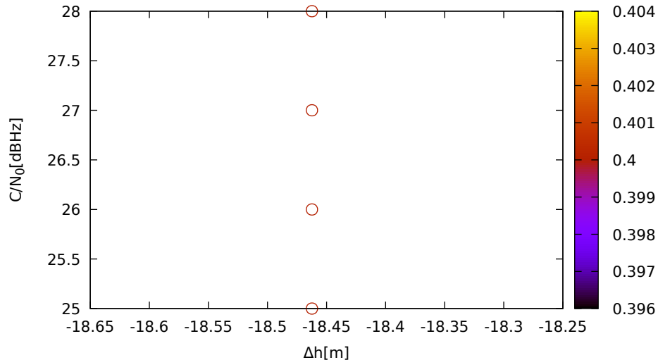
C/N 0 vs height (ublox9 (down) for R04 at L1)
