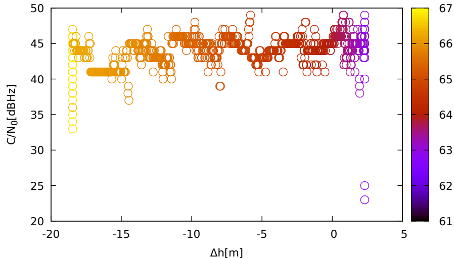
C/N 0 vs height (ublox9 (down) for R09 at L1)
