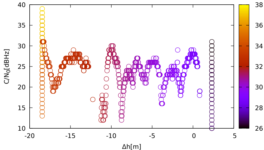
C/N 0 vs height (ublox9 (down) for R10 at L1)
