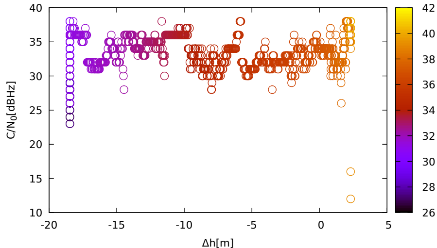
C/N 0 vs height (ublox9 (down) for R16 at L1)
