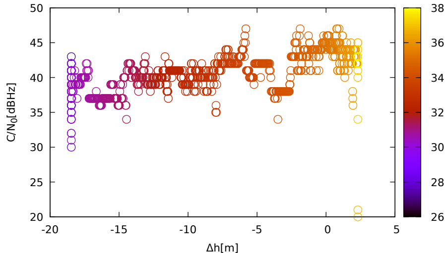
C/N 0 vs height (ublox9 (down) for R18 at L1)
