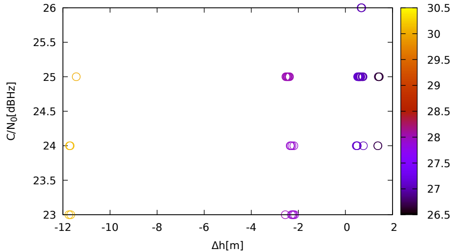
C/N 0 vs height (ublox9 (down) for R20 at L1)
