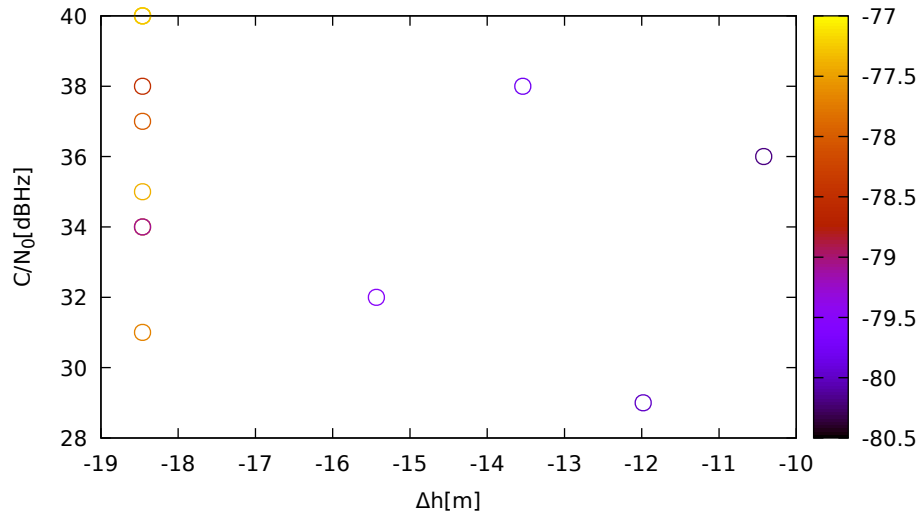
C/N 0 vs height (ublox9 (down) for R26 at L1)
