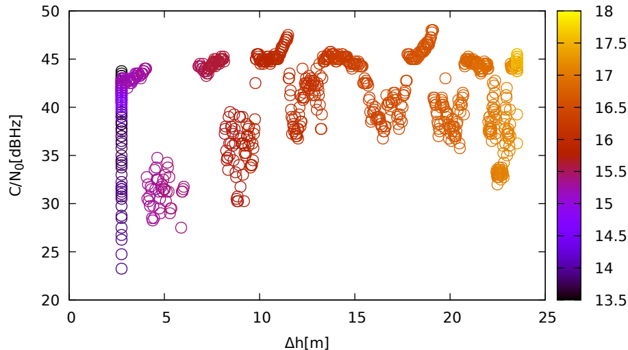
C/N 0 vs height (JavadLSA (up) for G05 at L1)
